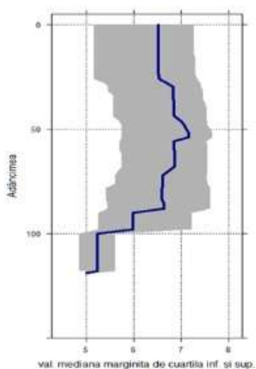
Fig. 10. pH variation for phaeozems
