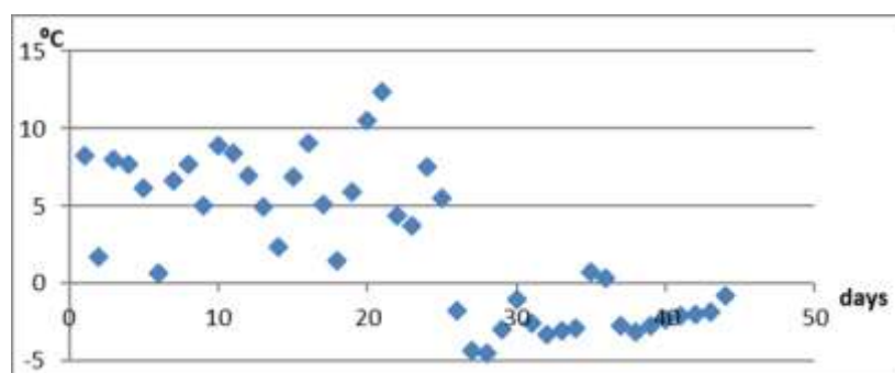
Fig.16. Daily average temperatures for the first 44 days of the vegetation period for 1998 (after Rocada)
