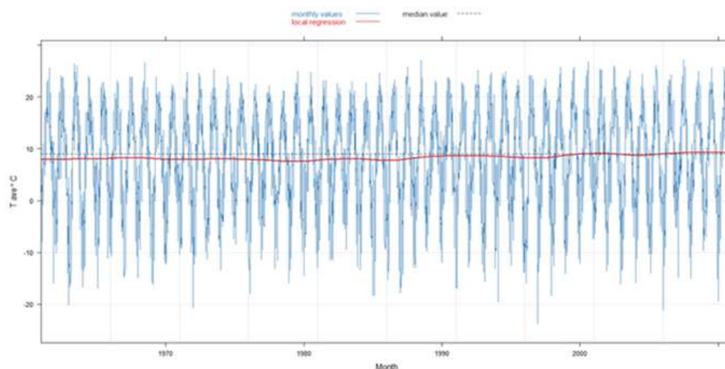
Fig.14. Monthly average temperatures (1961-2013, after Rocada)
