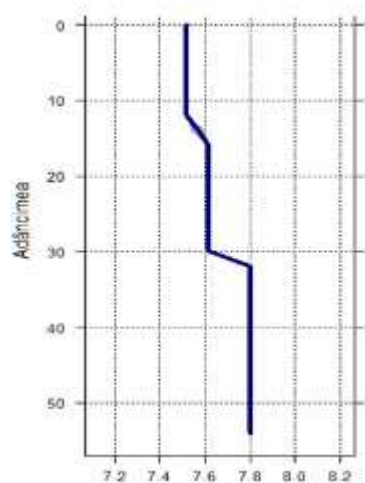
Fig. 12. pH variation for erodic anthrosol
