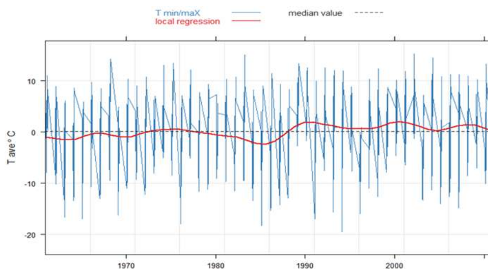
Fig.15. Multiannual average temperature for February and March (1961-2013, after Rocada)
