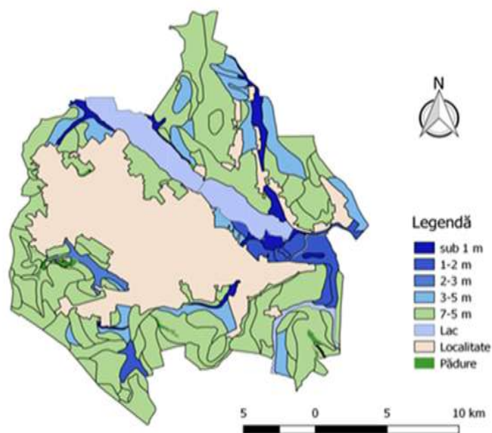
Fig.22. Ground water level
