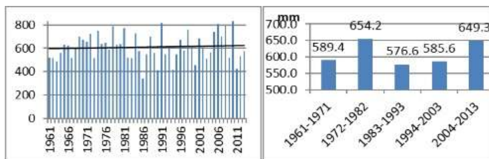
Fig.17. Multiannual average precipitations on decades (1961-2013, after Rocada)
