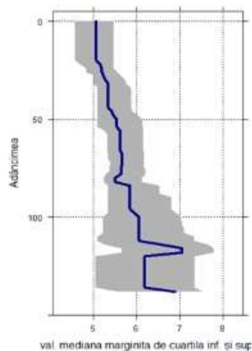
Fig. 11. pH variation for preluvosol
