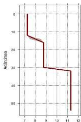
Fig. 13. \text{CaCO}_3 variation for erodic anthrosol
